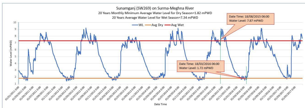
Figure 7-8: Sample Hydrograph of River Gauge Station at Sunamganj on Surma-Meghna River System
