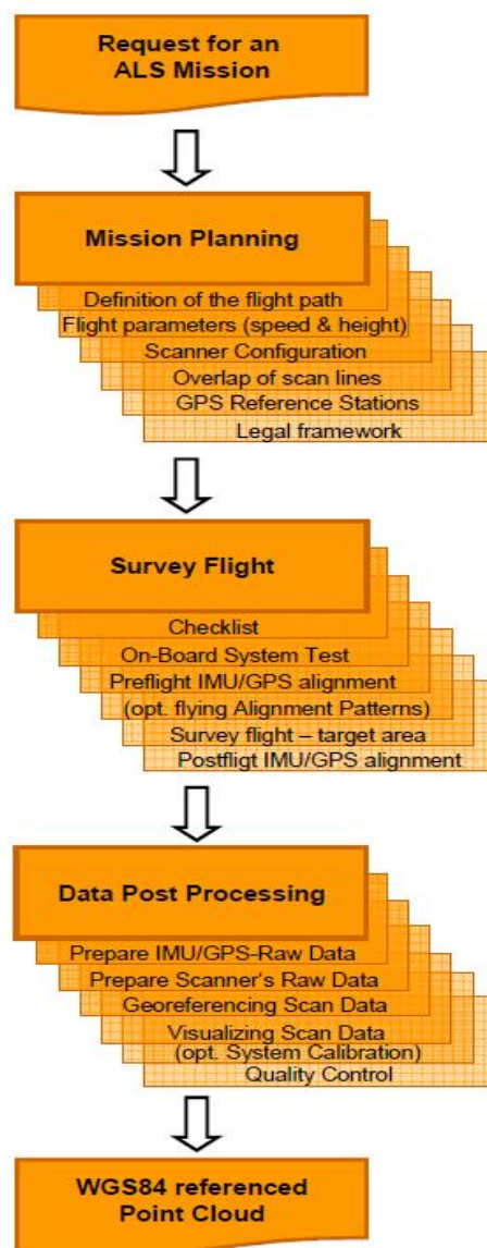
Figure 5-13: Flow Chart for LiDAR Survey and Image Processing
