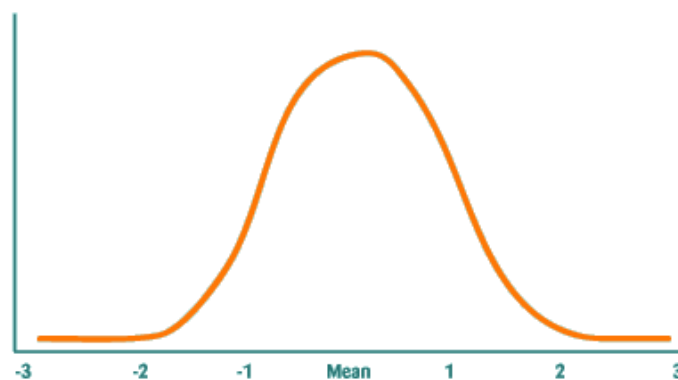
Figure 5-11: An Ideal Frequency Distribution Curve
