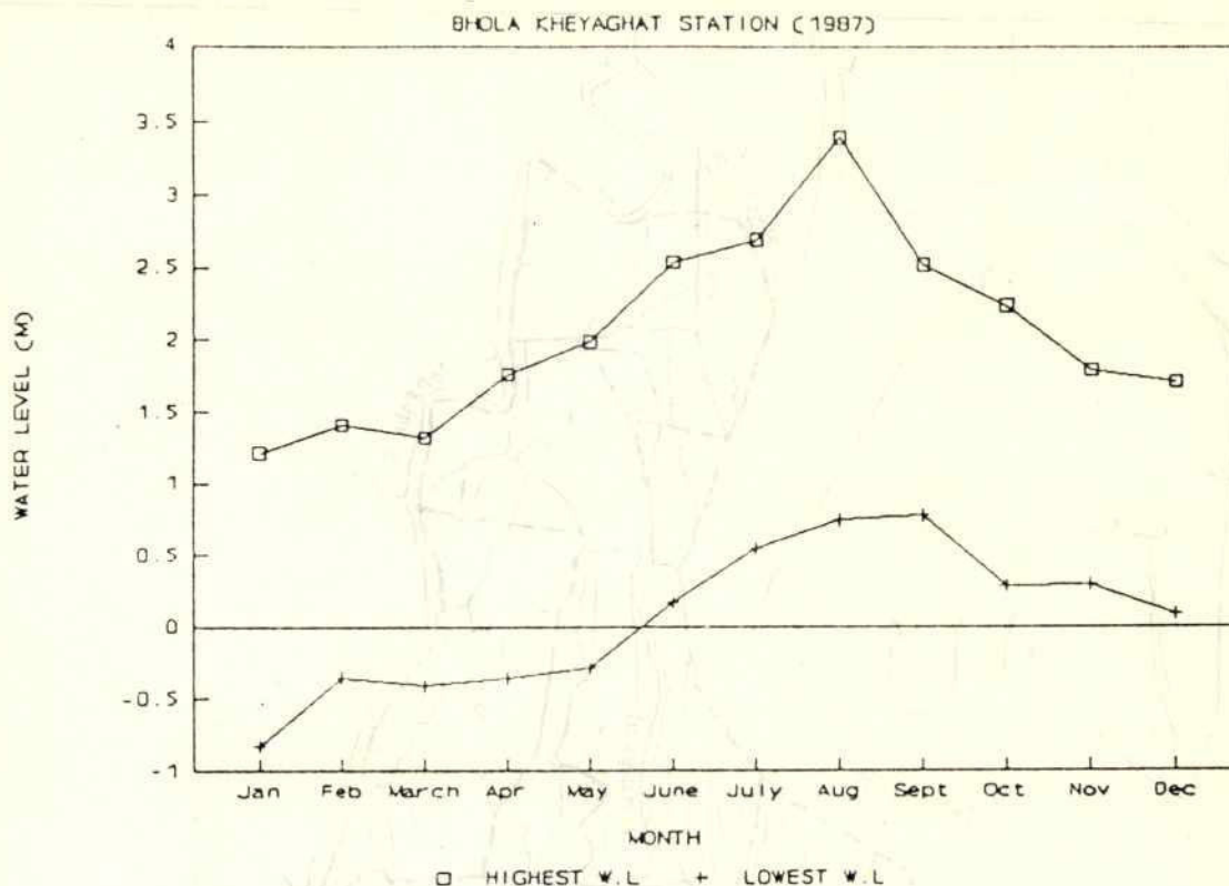
Figure 3.2 Example of annual water level fluctuations in the study area (data from Bhola Kheyaghat gauging station).
