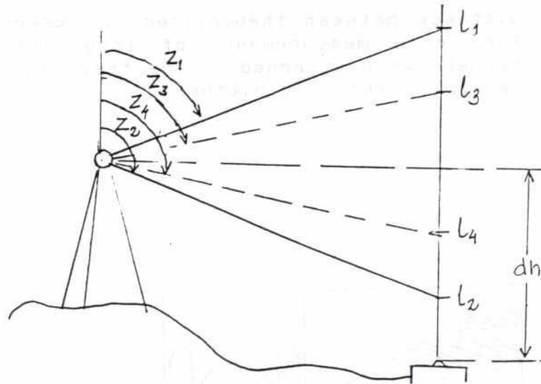
Picture 1. Height transfer from bench mark to theodolite.
