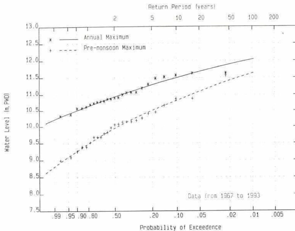
Gauge 135A Juni River (Continala Branch) at Continala General Extreme Value Distribution
