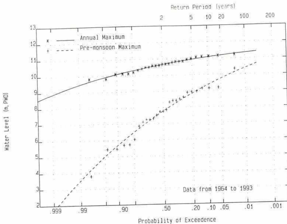
Gauge 252.1 Sarigowain River at Salutikan 3-Parameter Log Normal Distribution
