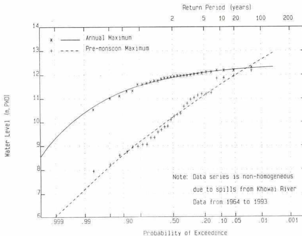
Gauge 138 Karangi River at Sofiabab 3-Parameter Log Normal Distribution
