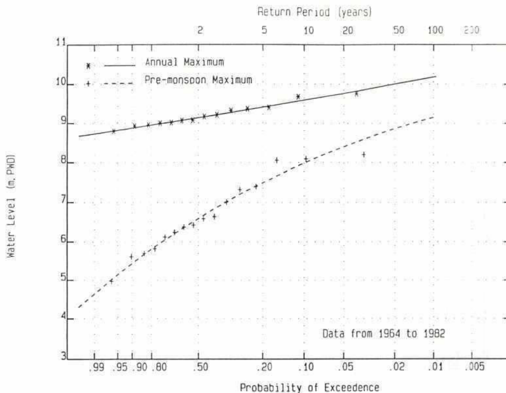
Gauge 175 Kushiyara River at Manumukh General Extreme Value Distribution
