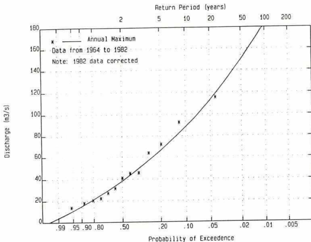
Gauge 227(R) Sutia Offtake from Old Brahmaputra River General Extreme Value Distribution
