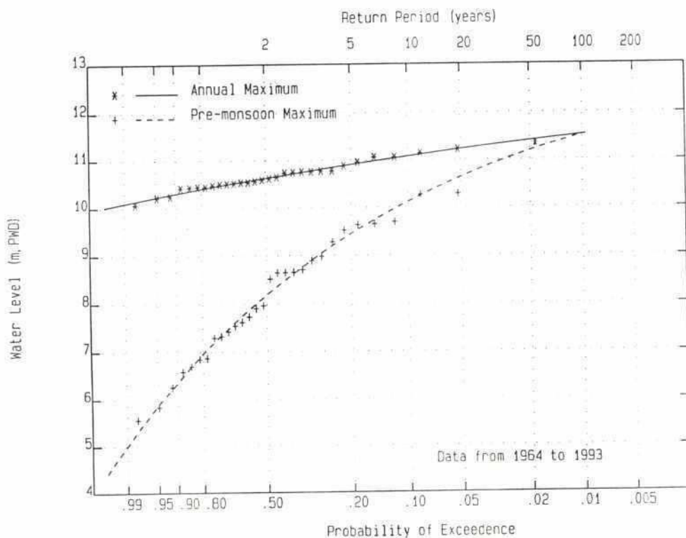
Gauge 174 Kushiya River at Fenchuganj General Extreme Value Distribution
