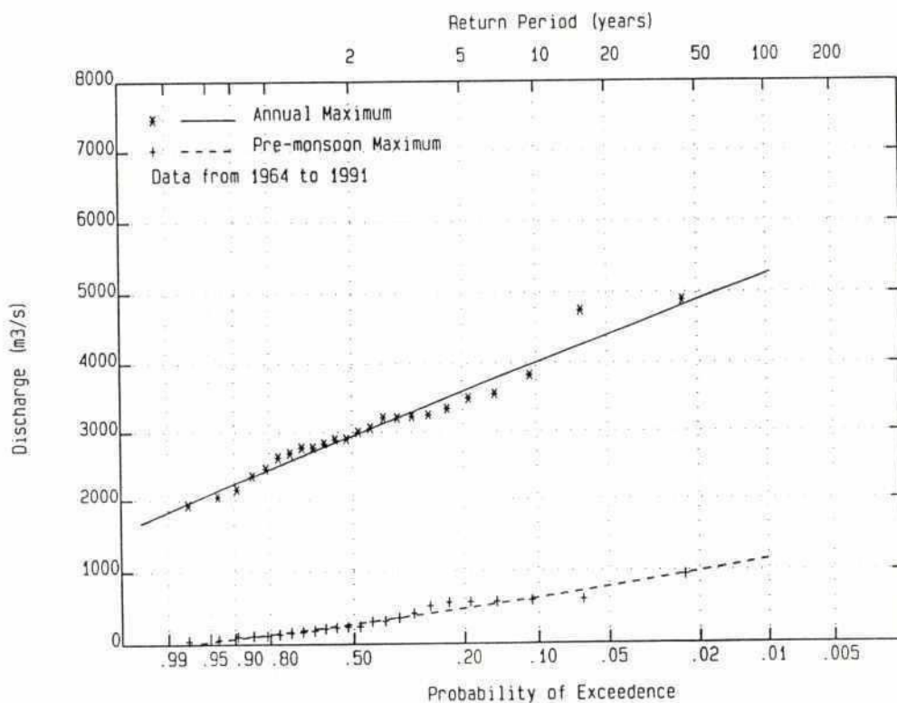
Gauge 228-5 Old Brahmaputra R. at Mymensingh (Nilukirchar) General Extreme Value Distribution
