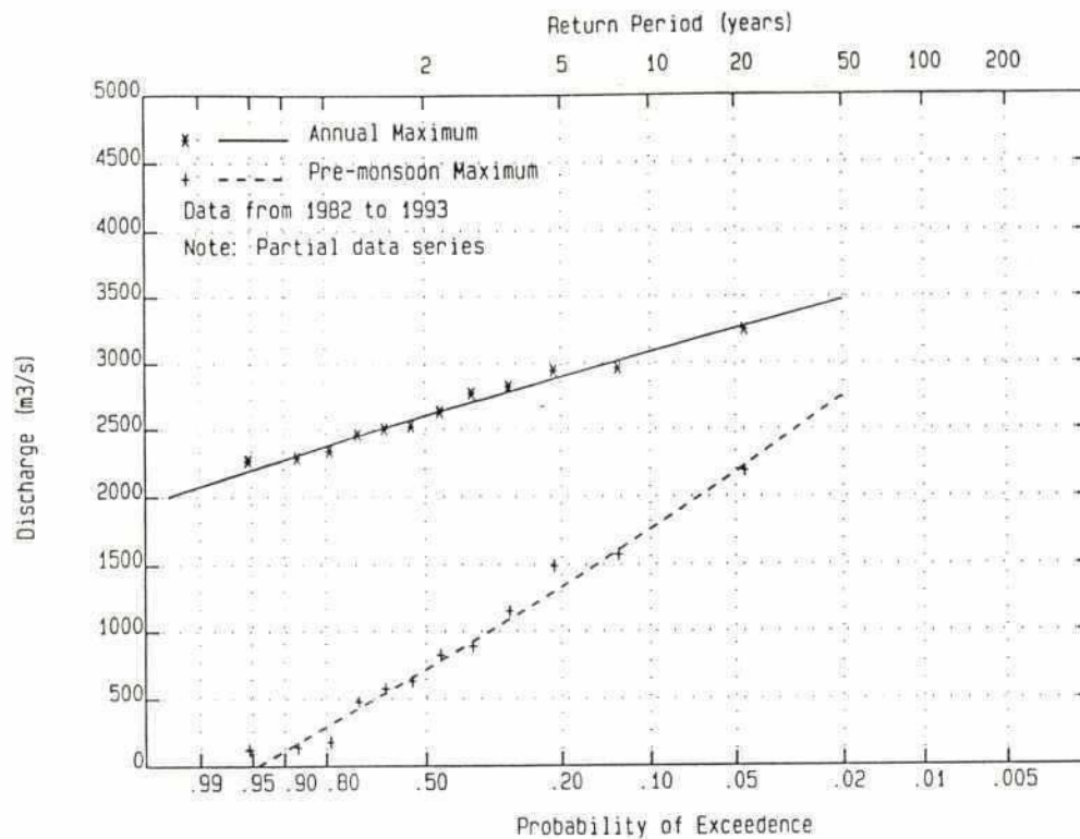
Gauge 173(R) Kushiya River at Sheola General Extreme Value Distribution
