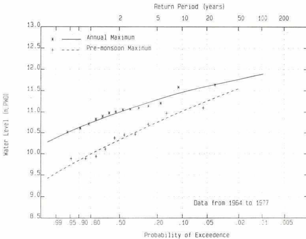
Gauge 135 Juni River (Juni Branch) at Continala General Extreme Value Distribution
