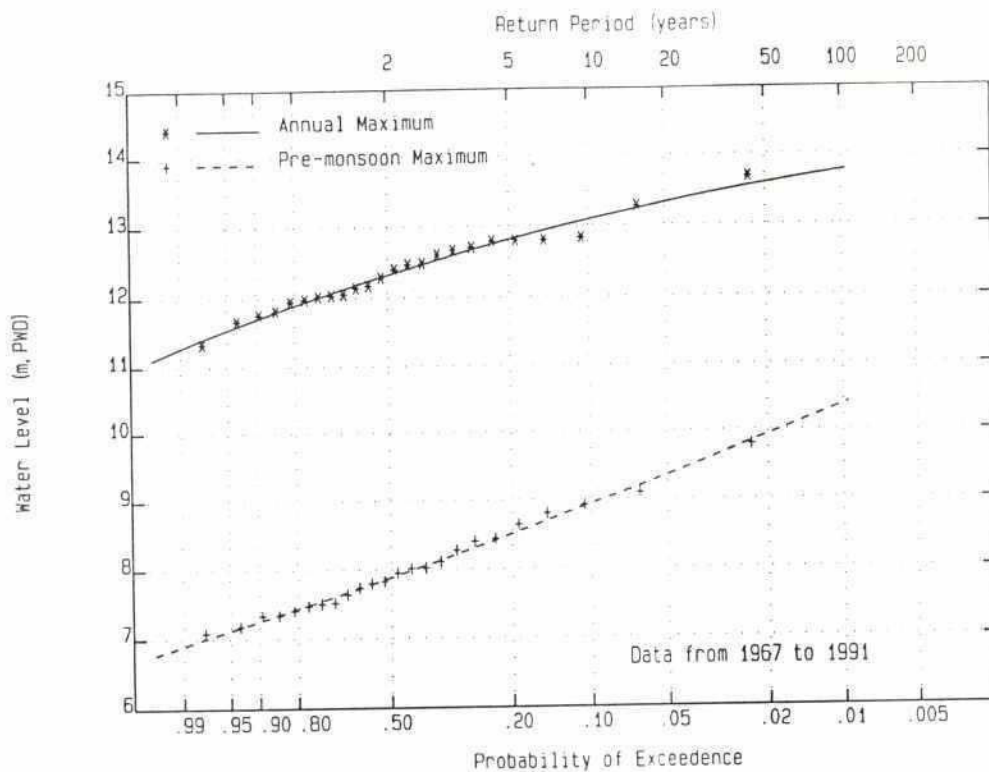
Gauge 228.5 Old Brahmaputra River at Mymenshingh General Extreme Value Distribution
