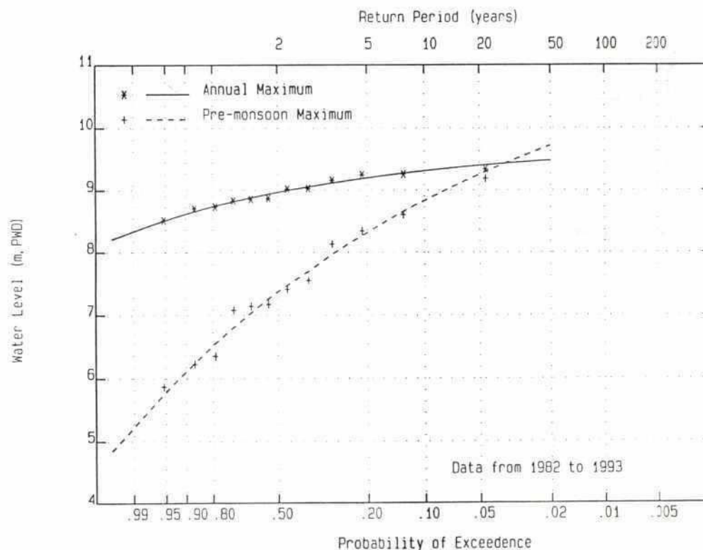
Gauge 175.5 Kushiyara River at Sherpur General Extreme Value Distribution
